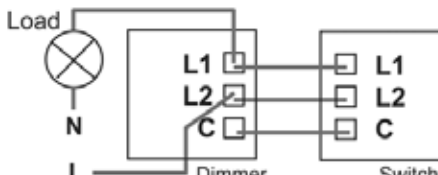
Figure 3. Using a 2-way Dimmerswitch.
