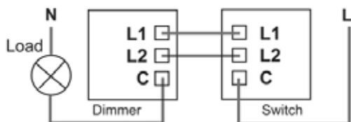
Figure 2. Using a 2-way Dimmerswitch.
